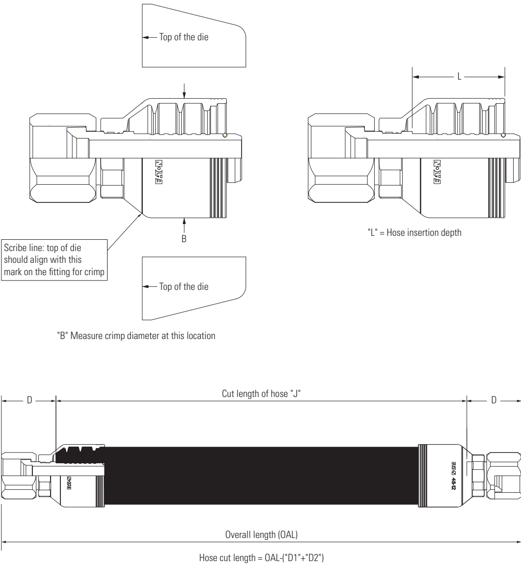
L Dimension
